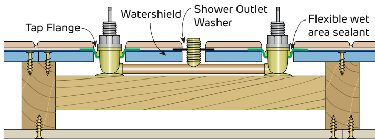
FIGURE 53 Alternative Plumbing Penetrations
