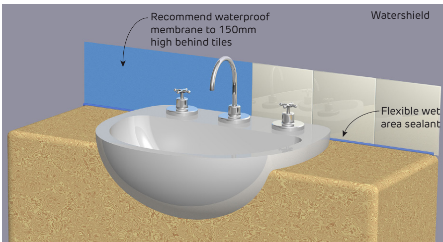
FIGURE 39 Basin
