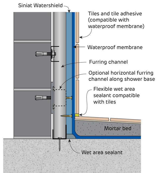
FIGURE 48 Shower over Masonry Wall Class 3 membrane shown - Section
