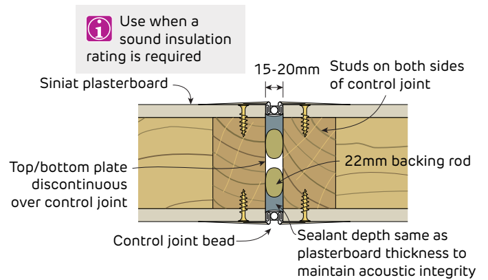
FIGURE 34 Wall Control Joint Plan
