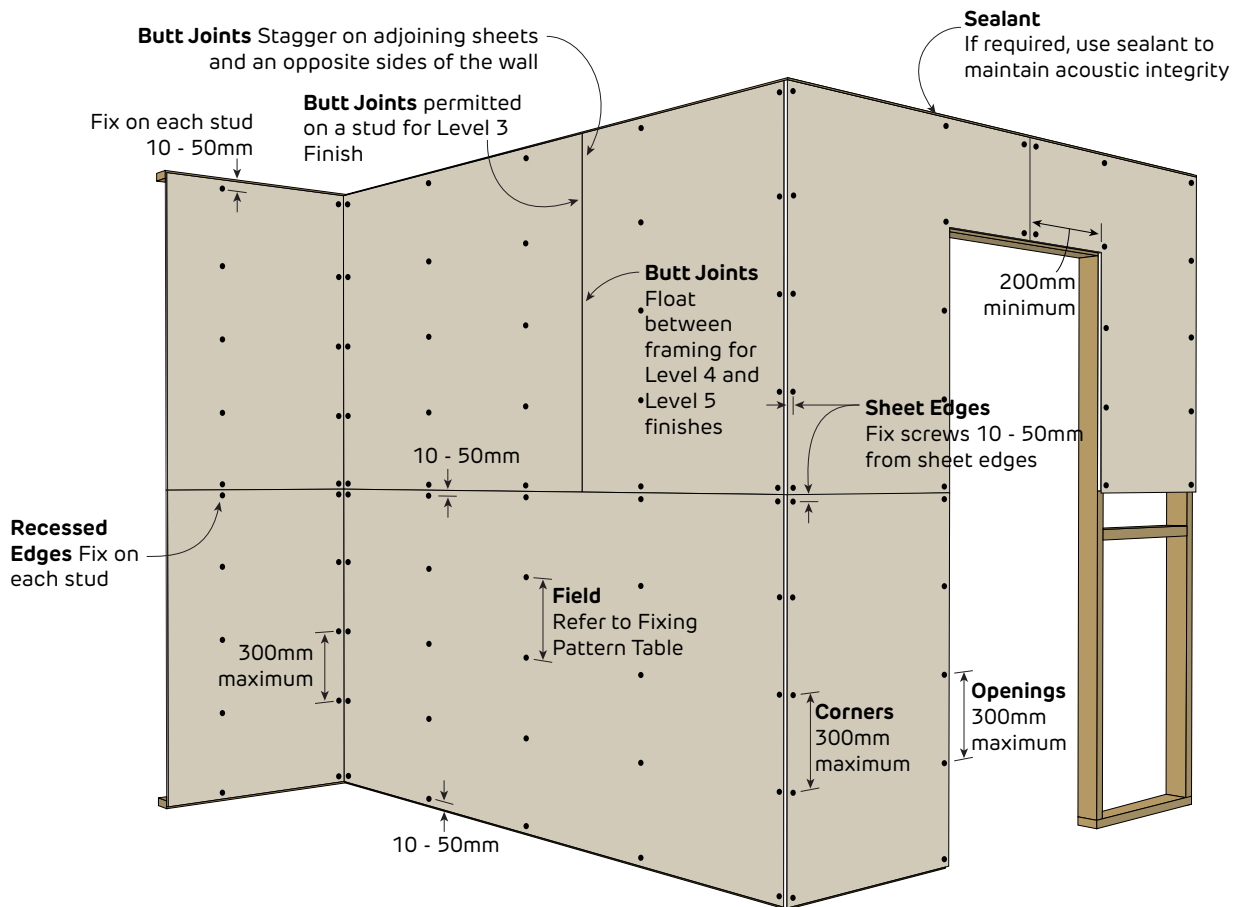
FIGURE 27 Internal Wall - 1 Layer Horizontal Fastener Only Method
