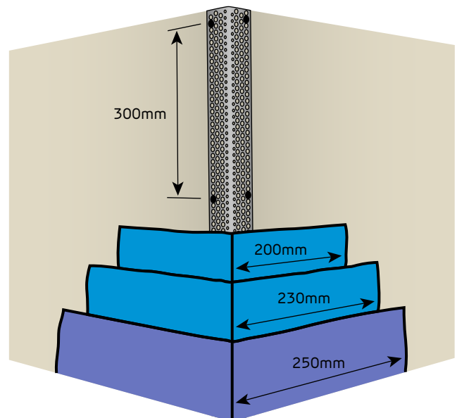
FIGURE 66 External Corner
