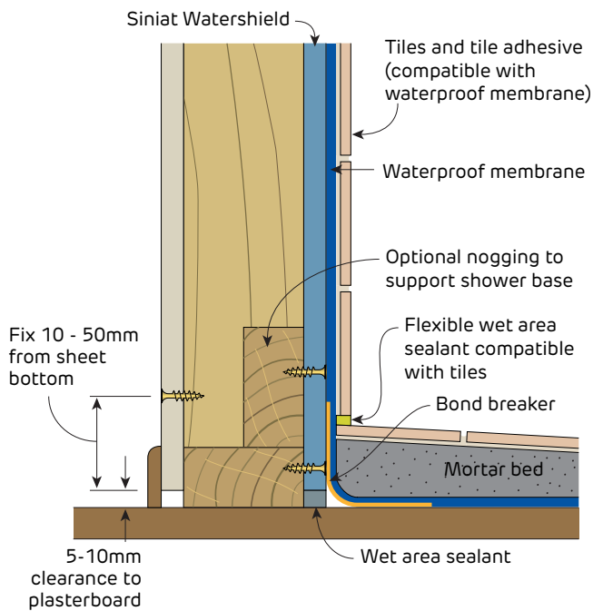
FIGURE 45 Shower Base Shower over particleboard flooring Class 2 membrane shown - Section
