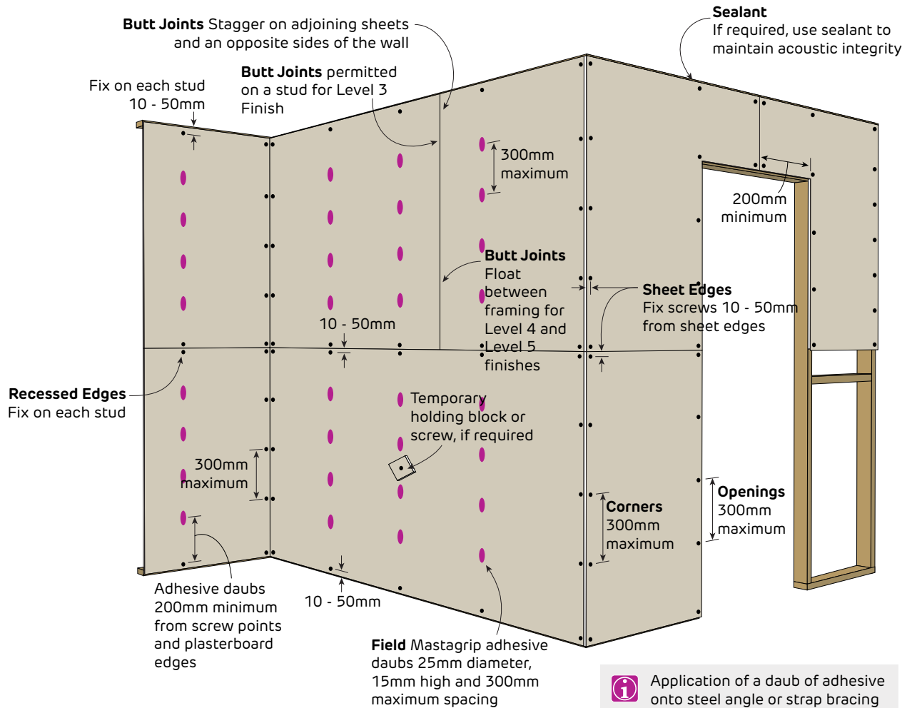
FIGURE 26 Internal Wall - 1 Layer Horizontal Fastener and Adhesive Method
