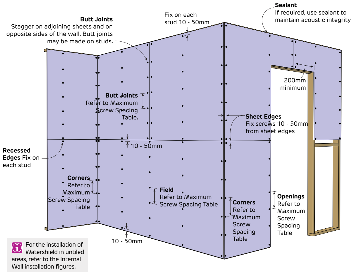
FIGURE 43 Watershield in Tiled Areas - 1 Layer Horizontal Screw Only Method
