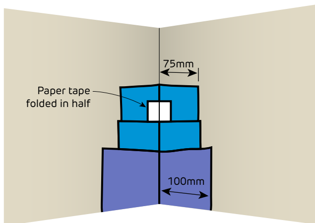
FIGURE 65 Internal Corner
