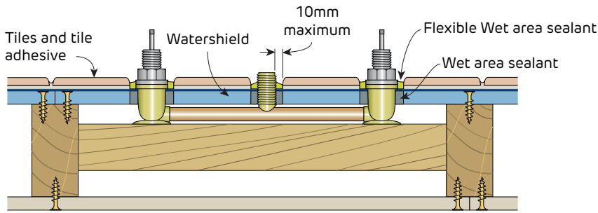
FIGURE 52 Plumbing Penetrations
