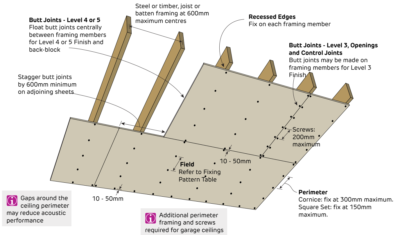
FIGURE 7 Internal Ceiling - 1 Layer Fastener Only Method
