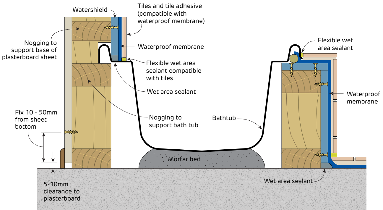
FIGURE 51 Bathtub Section
