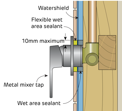
FIGURE 54 Plumbing Penetration
