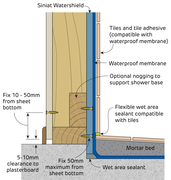
FIGURE 46 Shower Base Shower with concrete slab drop down Class 3 membrane shown - Section
