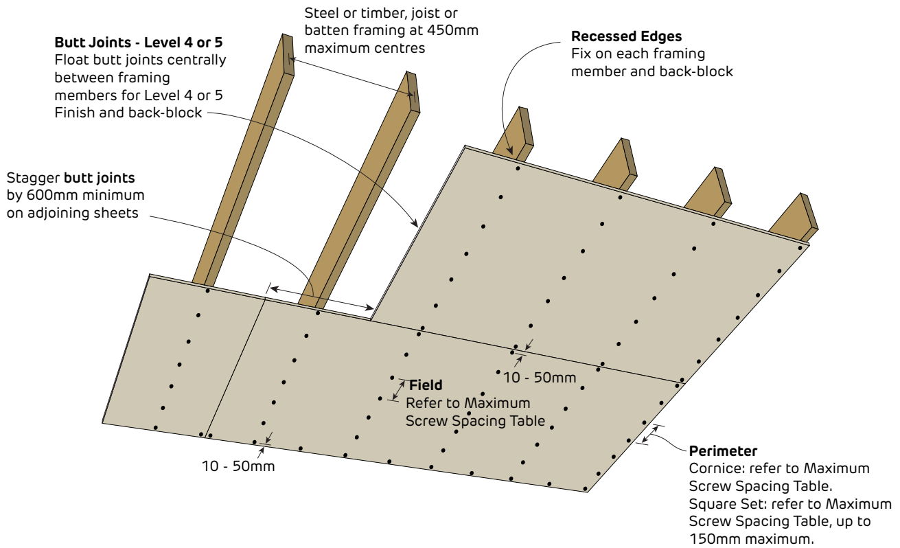
FIGURE 20 External Ceiling - 1 Layer Screw Only Method
