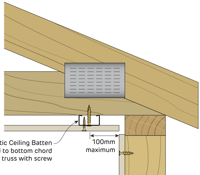
FIGURE 12 Direct Fix Ceiling to Roof Truss 16mm Domestic Batten fixed directly to trusses Section
