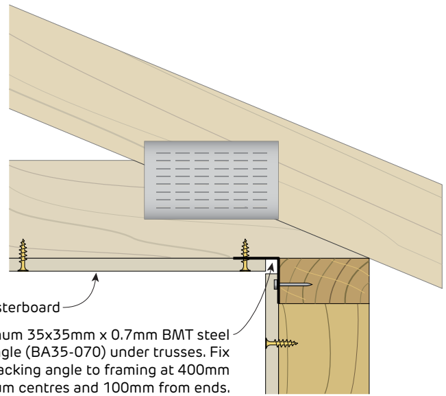
FIGURE 10 Perimeter Framing for Plasterboard Section
