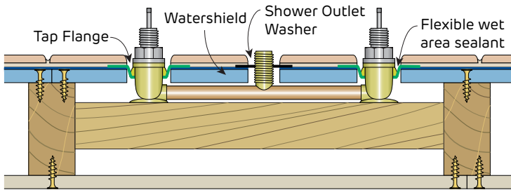
FIGURE 54 Alternative Plumbing Penetrations Propriety tap flange and shower outlet washer Plan
