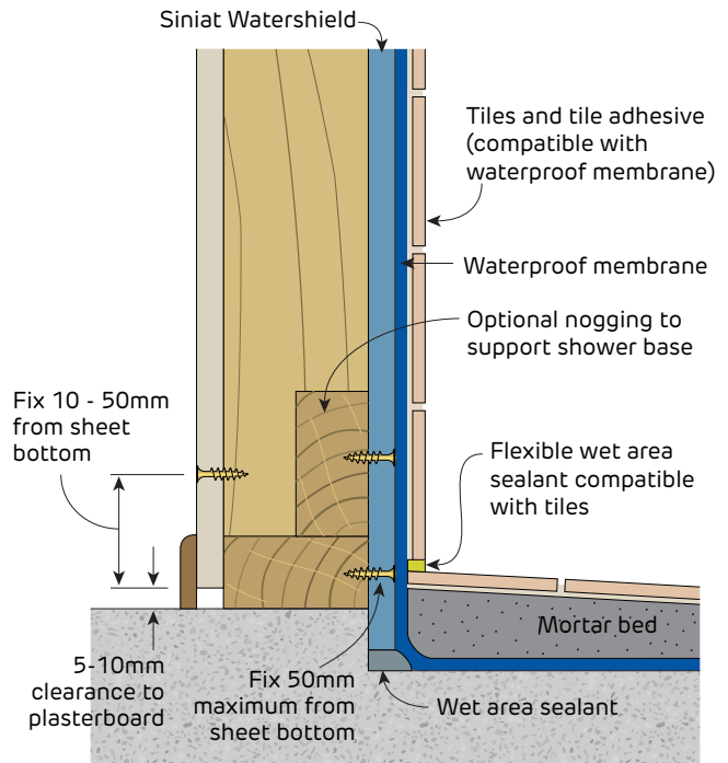
FIGURE 47 Shower Base Shower with concrete slab drop down Class 3 membrane shown - Section
