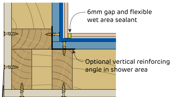
FIGURE 50 Shower Corner Plan
