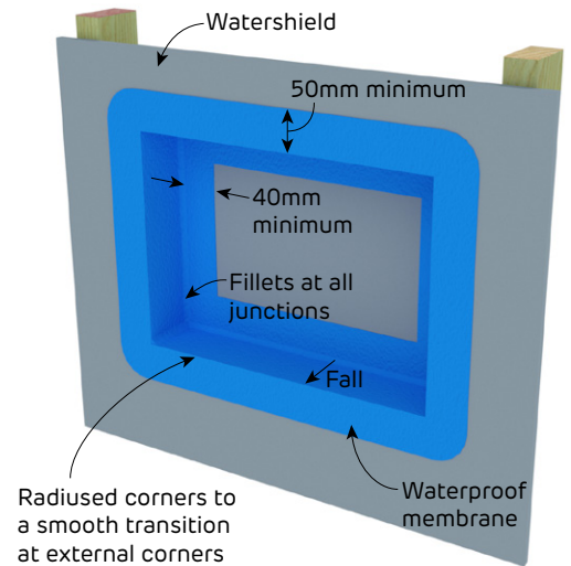
FIGURE 43 Shower Niche
