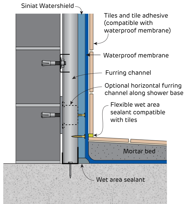
FIGURE 49 Shower over Masonry Wall Class 3 membrane shown - Section
