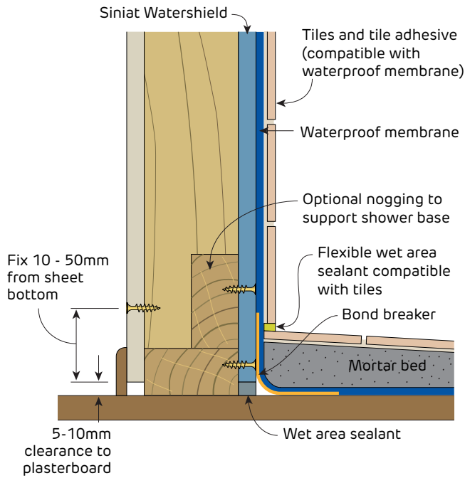
FIGURE 46 Shower Base Shower over particleboard flooring Class 2 membrane shown - Section
