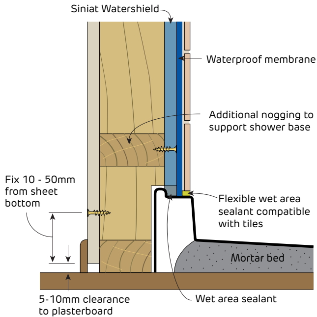
FIGURE 48 Shower Base Pre-formed shower tray - Section
